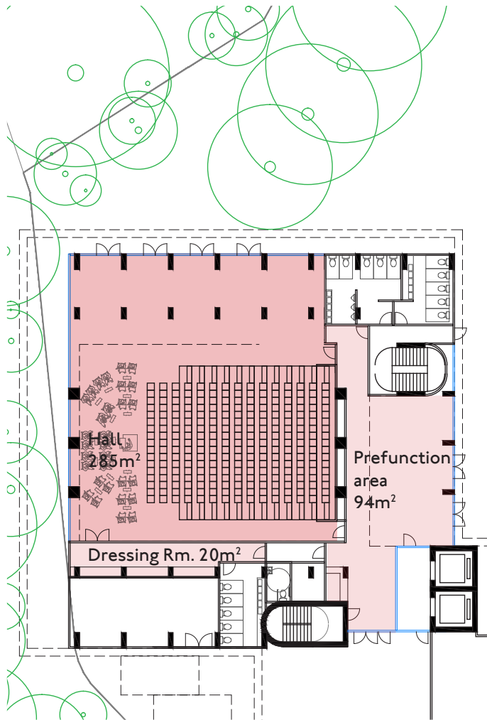
Concert 255 seats (17 x 15 rows)
